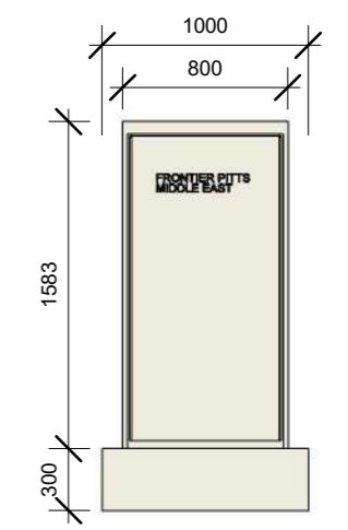
DETAIL A CABINET CONTROL POSITION TO SUIT SITE
